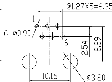
PC BOARD LAYOUT THICKNESS=1.6mm
